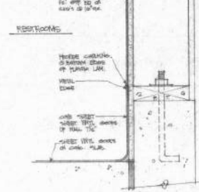
18 WOMEN'S RESTROOM 110
