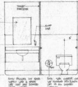
16 WOMEN'S RESTROOM 108
