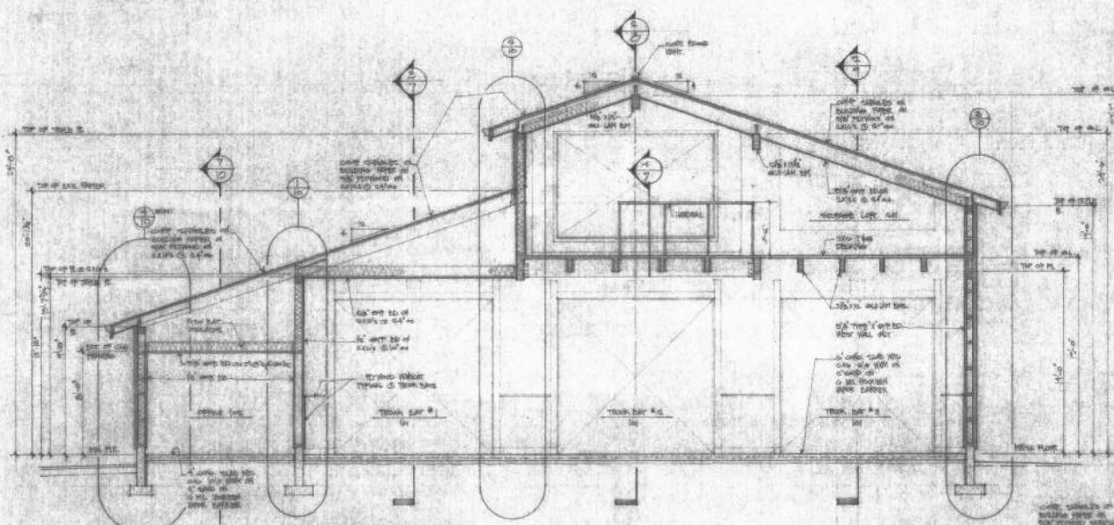
1 BUILDING SECTION
