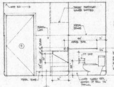
15 WOMEN'S RESTROOM 107
